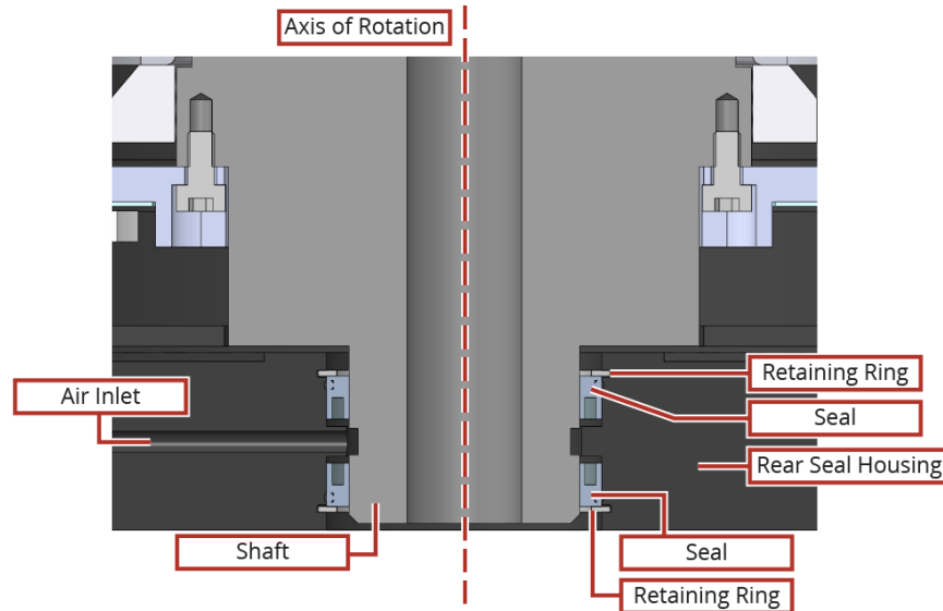
Figure 4-5: Cross-section View of Rear Seal Showing Seal Orientations
