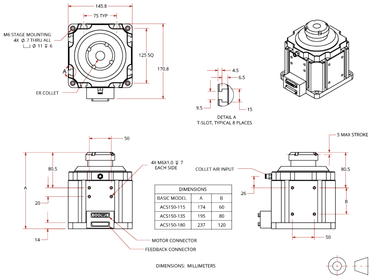
Figure 2-2: ACS150 (-ER Chuck Style) Dimensions
