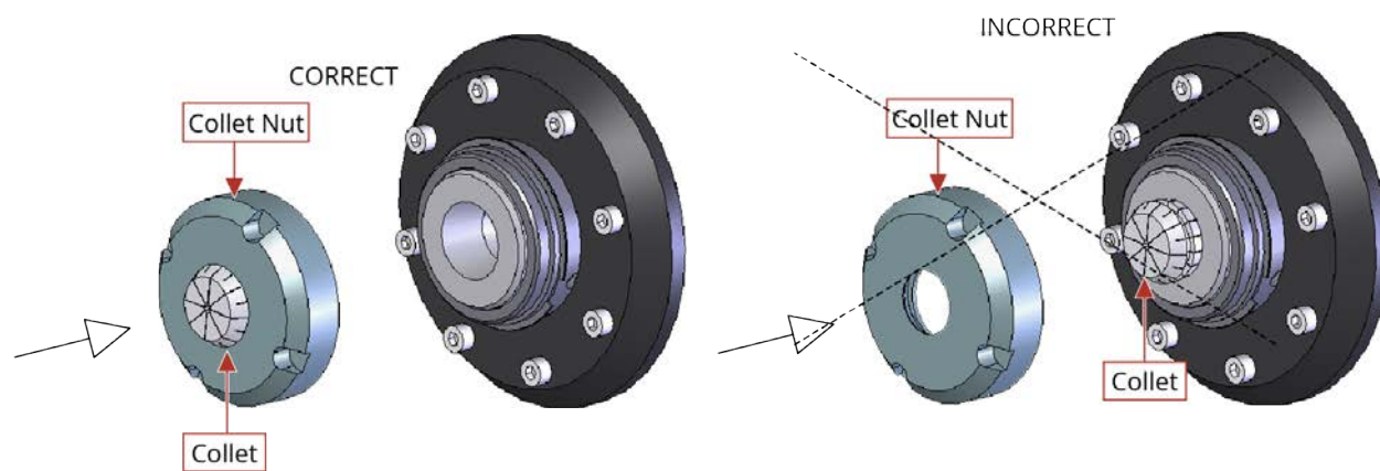
Figure 2-8: Installation Procedure for Collet
