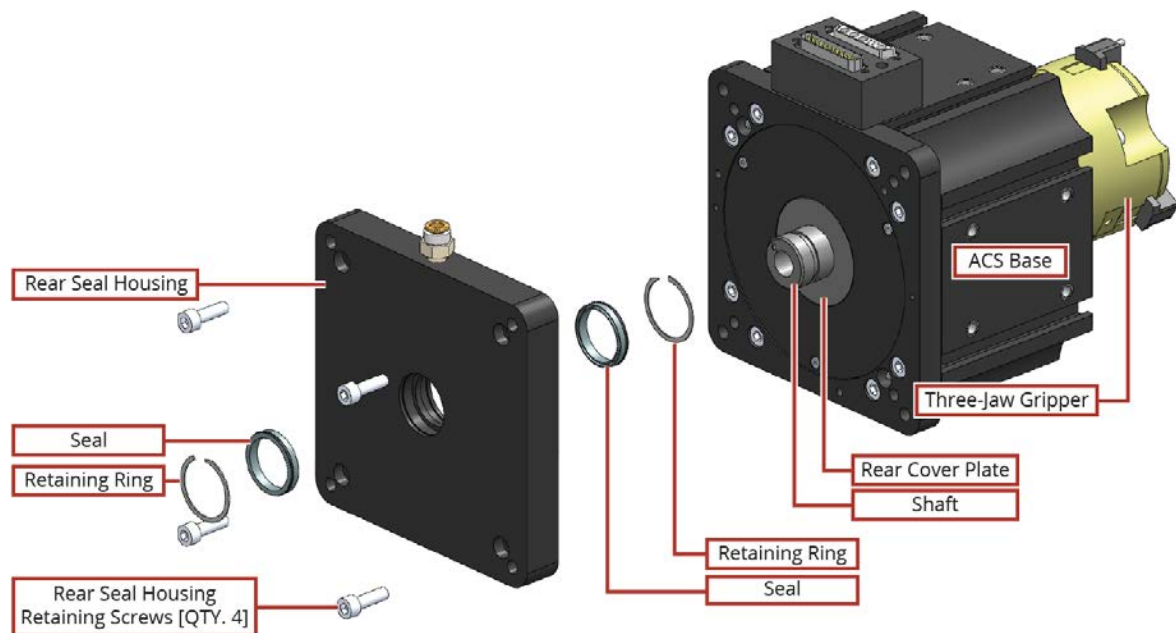
Figure 4-4: Exploded Drawing of Rear Seal Components
