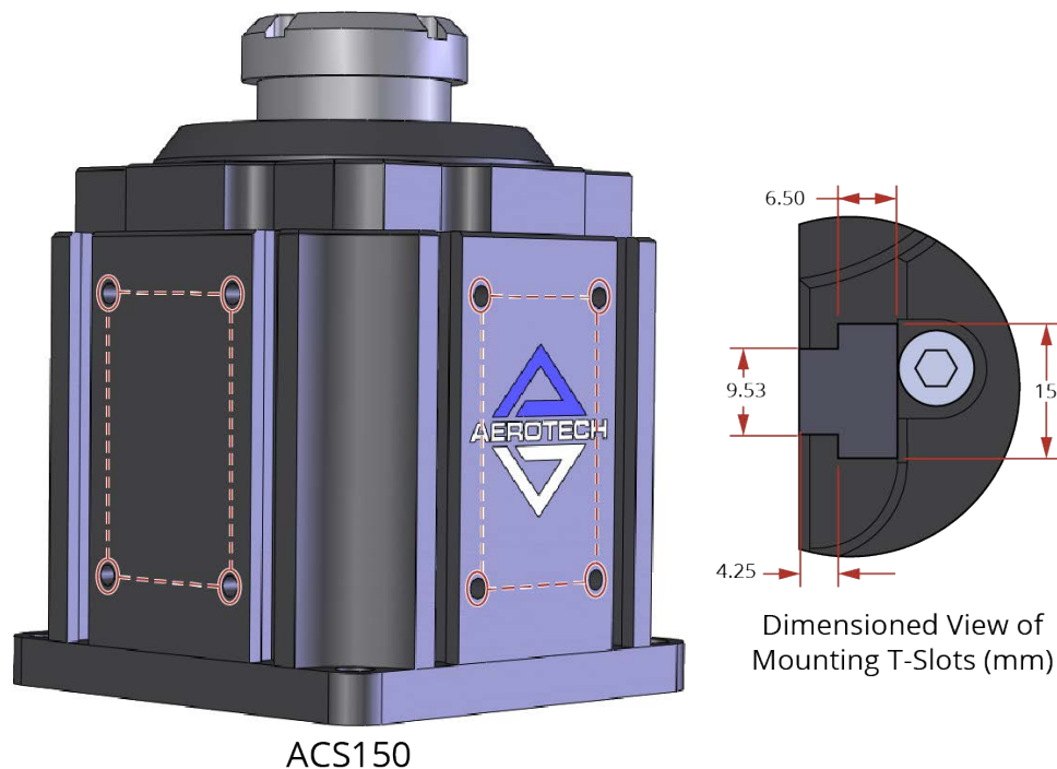
Figure 2-6: Typical ACS150 Stage Showing Side Mounting Holes and T-Slot Detail
