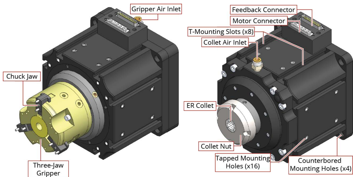
Figure 1-1: ACS Rotary Stage with Callouts
