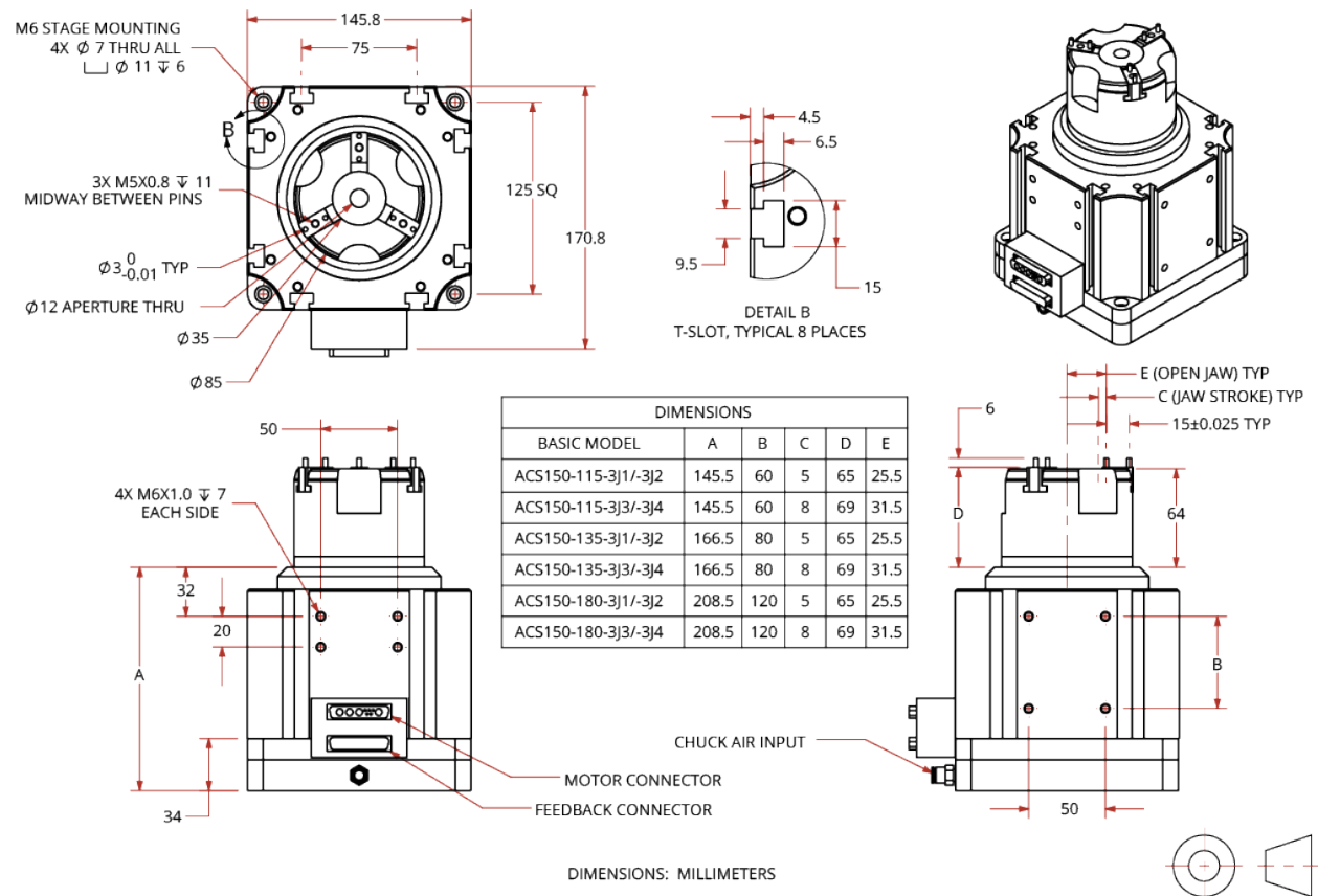
Figure 2-3: ACS150 (-3J Chuck Style) Dimensions
