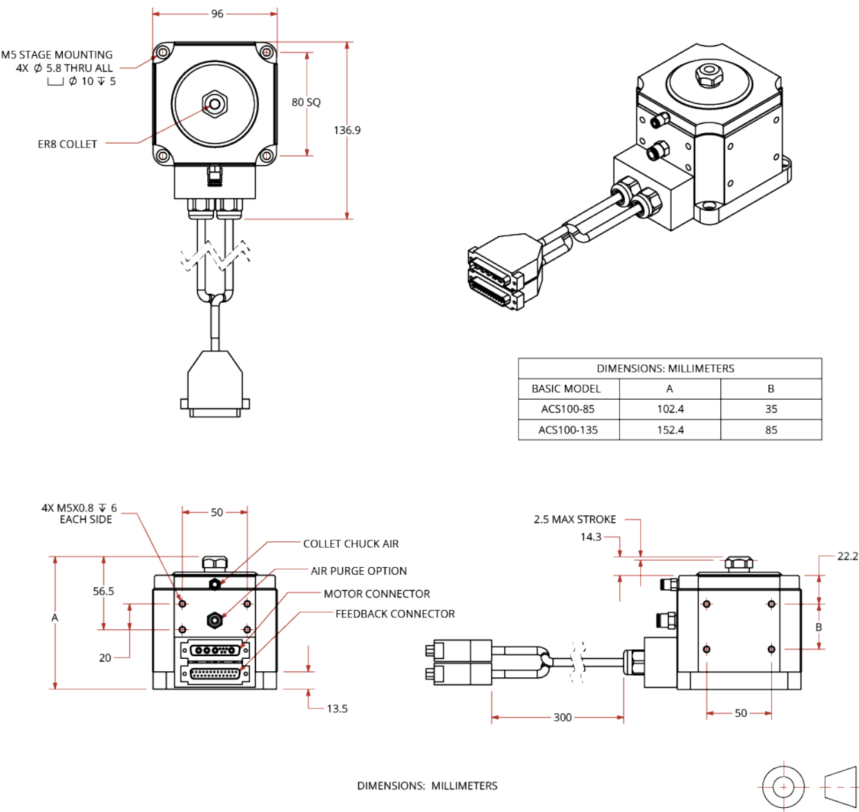
Figure 2-1: ACS100 Dimensions
