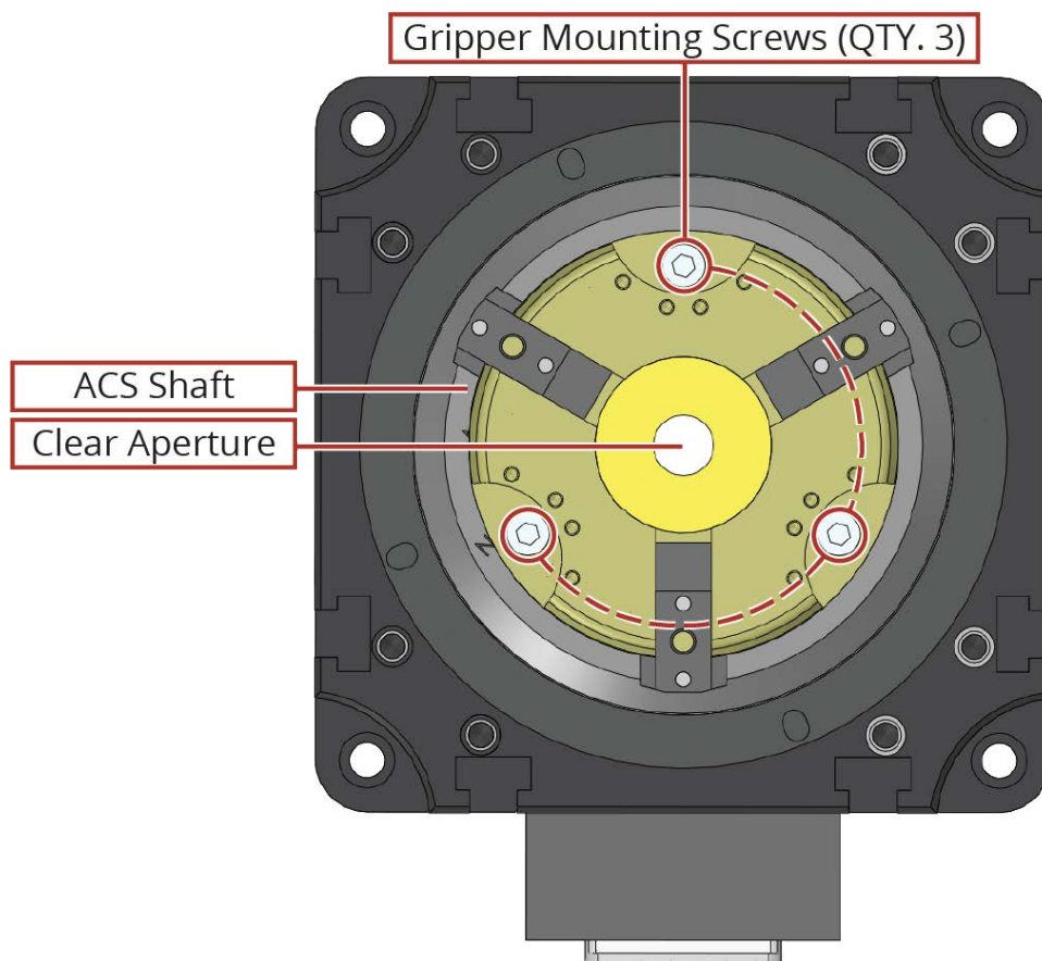
Figure 2-11: Mounting Holes for Three-Jaw Gripper
