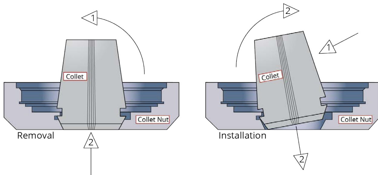
Figure 2-7: Schematic of Collet Insertion Into and Removal From Collet Nut
