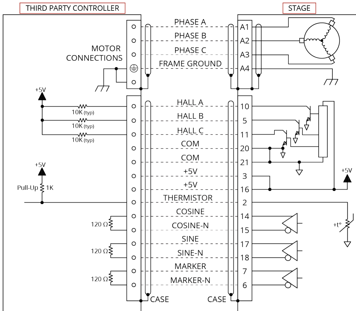
Figure 3-1: Motor and Feedback Wiring (ACS100 -CN1)
