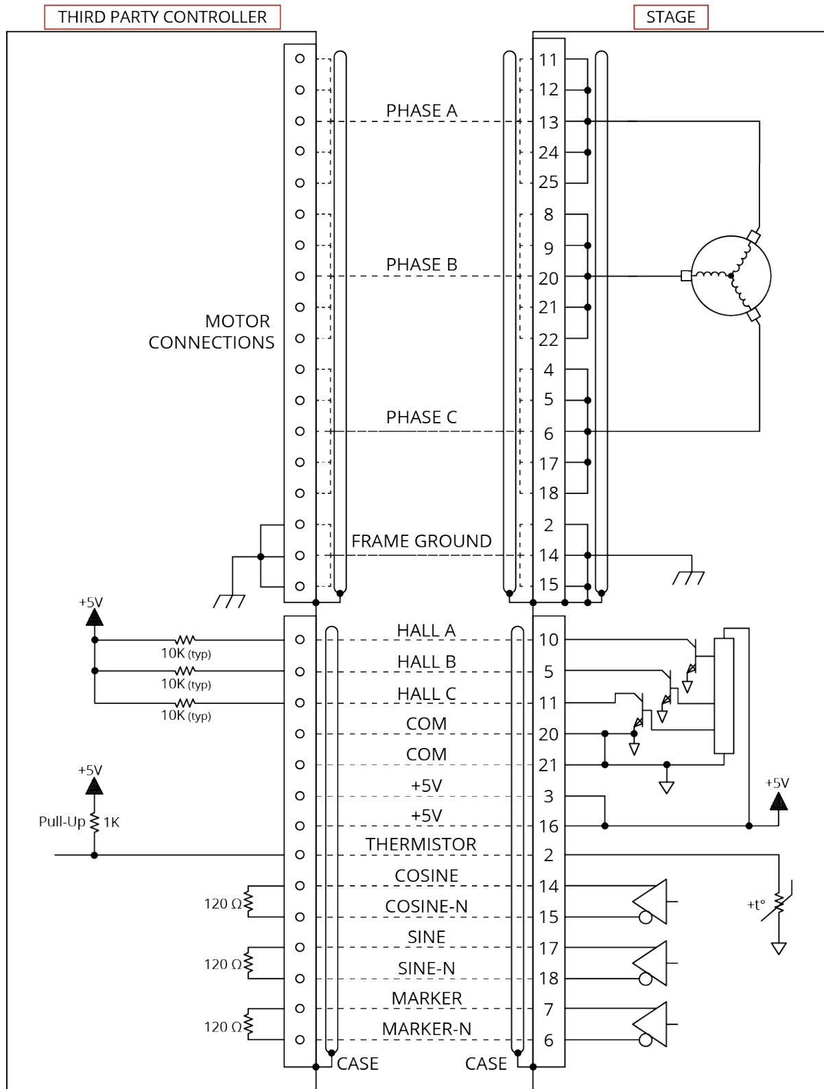
Figure 3-2: Motor and Feedback Wiring (ACS100 -CN2)
