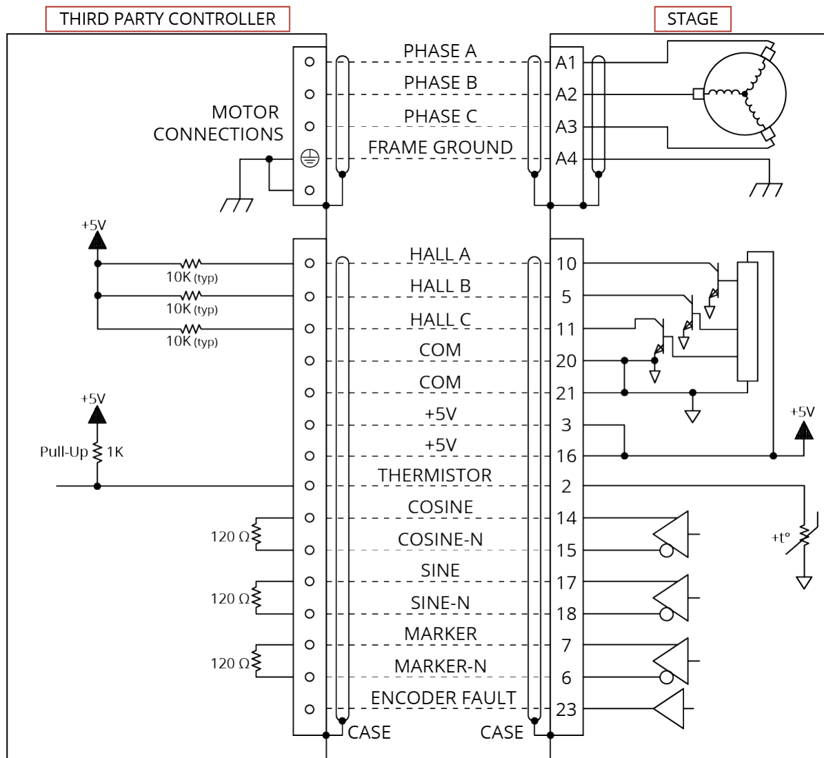
Figure 3-3: Motor and Feedback Wiring (ACS150 and ACS200)
