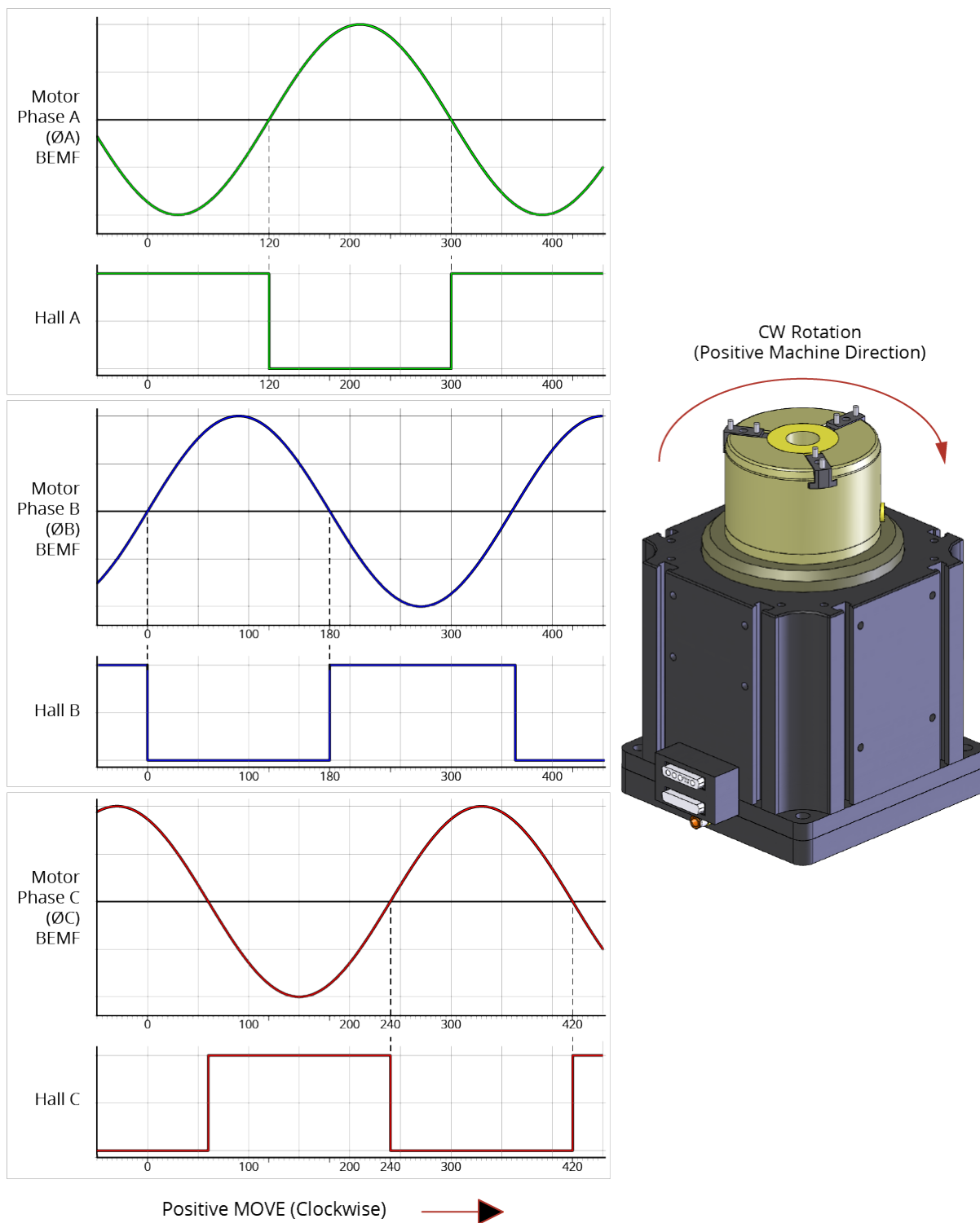
Figure 3-5: Hall Phasing
