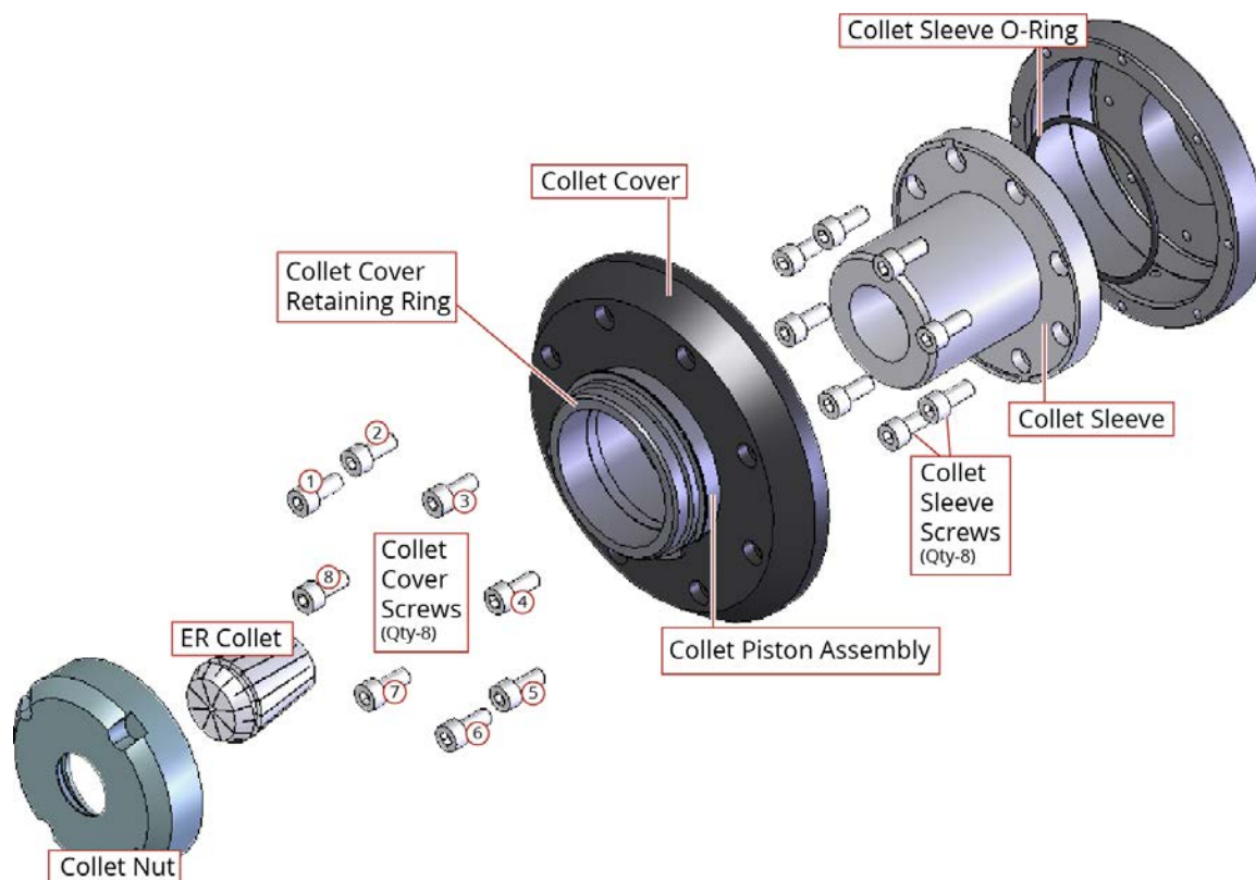
Figure 2-9: Collet Assembly Exploded View
