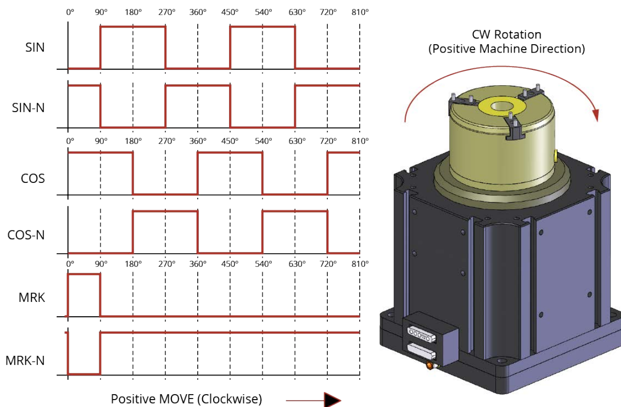
Figure 3-7: Encoder Phasing Reference Diagram (Standard)
