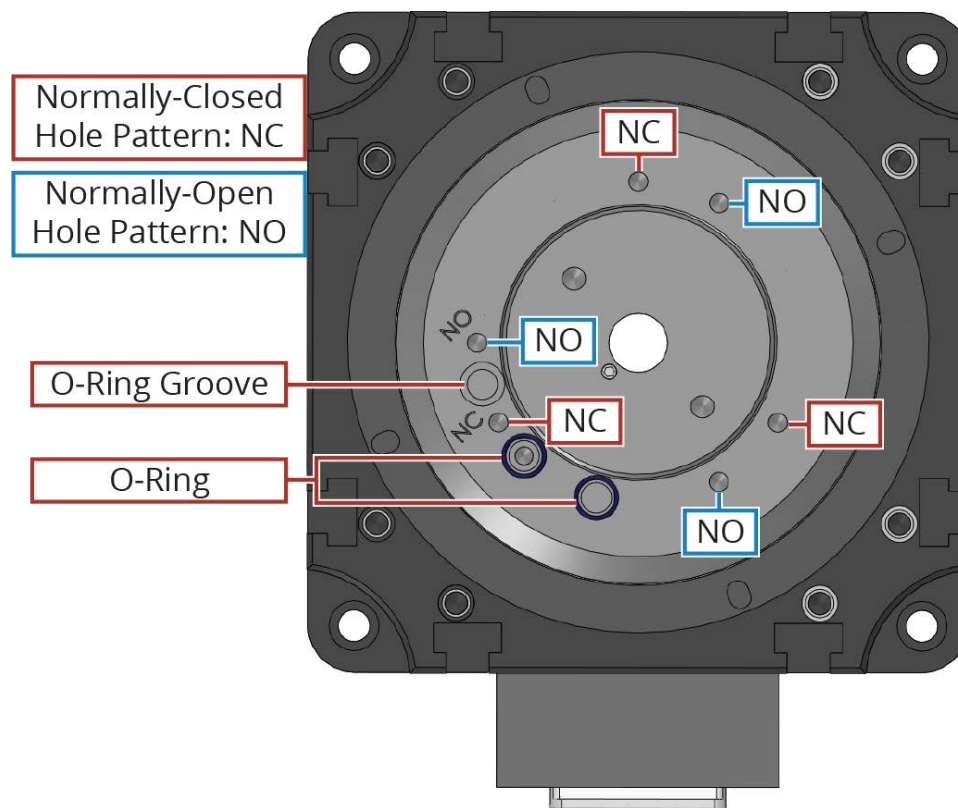
Figure 2-10: Gripper Mounting Hole Locations in ACS Shaft
