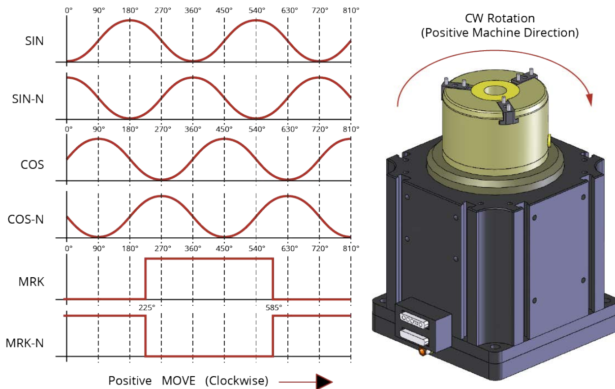
Figure 3-6: Analog Encoder Phasing Reference Diagram
